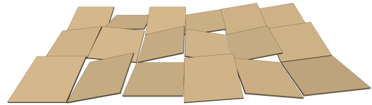
Fig. 5: Testbed of inclined support regions used during the benchmarking tests of our planning method. The testbed is organized in three rows, each with six supports. Each support is 40 cm \times 40 cm and has an inclination of either 10° or 15°.
