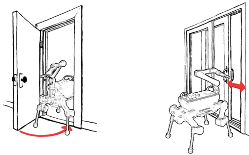
Fig. 8: Left: Door rotating over its hinges as a pivot point. Right: Door sliding back and forth on a frame.
